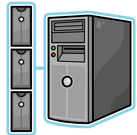
Digital database
