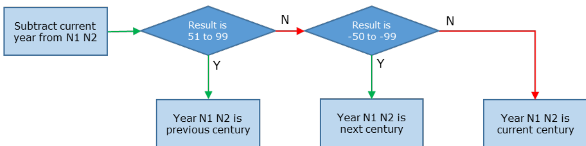
Figure 7.12-1. Determination of century
