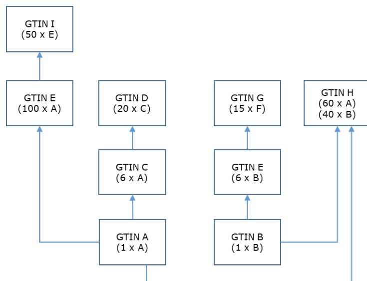
Figure 7.6.2-1. Extended example of trade item hierarchy
